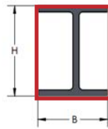
4 Sided Protection: Heated Perimeter = (2 \times H) + (2 \times B)
